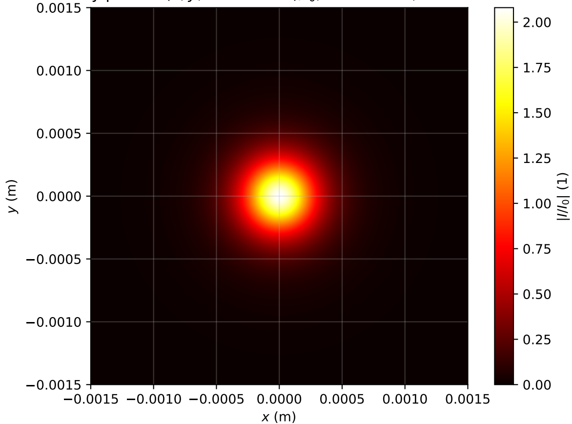
Intensity profile I(x, y, z = 1.911m)/I_0 , P_{in}=1.0P_{cr} , artificial time
